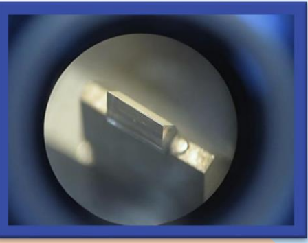
⑨ Finishing It was finished the diamond knife by using natural stone. Specification; Ultra / width 2.0 mm / angle with 45°
